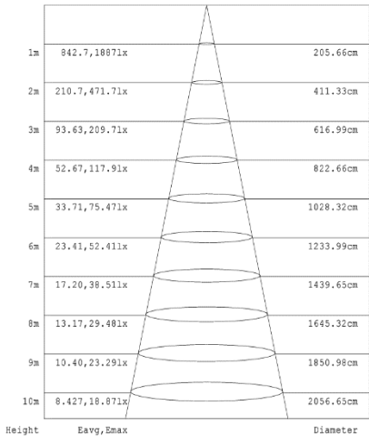
Cone Illuminance Diagram
